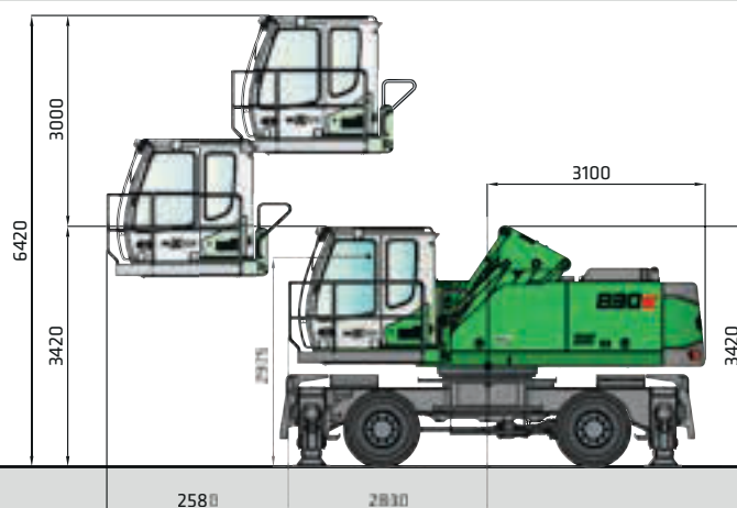
830 M with cab type E300/260 (option), can be elevated and moved forward hydraulically
